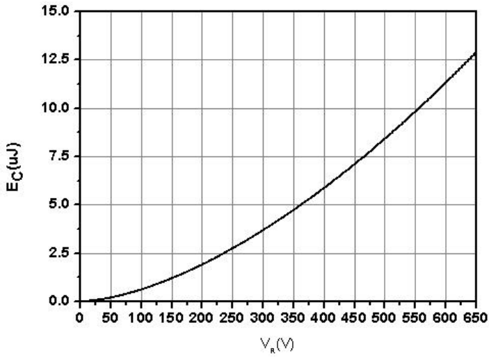
Fig.5-Capacitance Stored Energy
