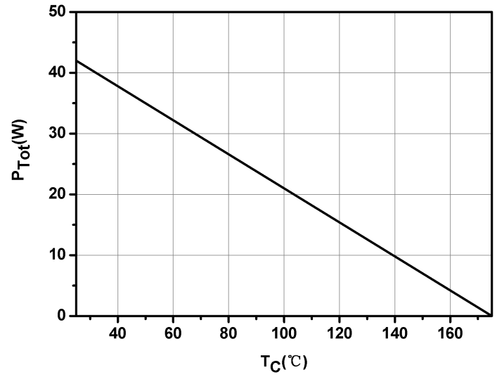
Fig.6-Power Derating
